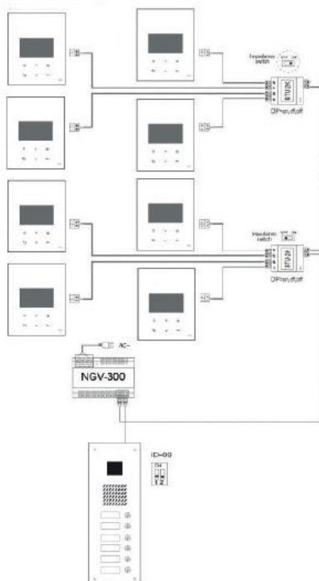
Connection Diagramm
